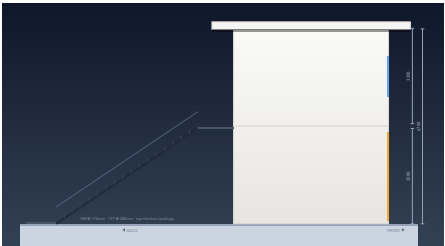
▶ SIDE / END – 1 M CANOPY PROJECTION · STAIR · HEIGHTS (MM)
